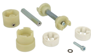
HRP9133 RIELLO DRIVE/COUPLING (RL28/38) (3003758)
